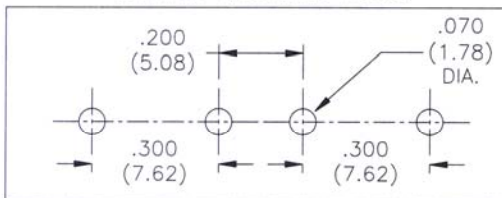
TYPICAL 9 VOLT BATTERY CONTACT MOUNTING HOLES
